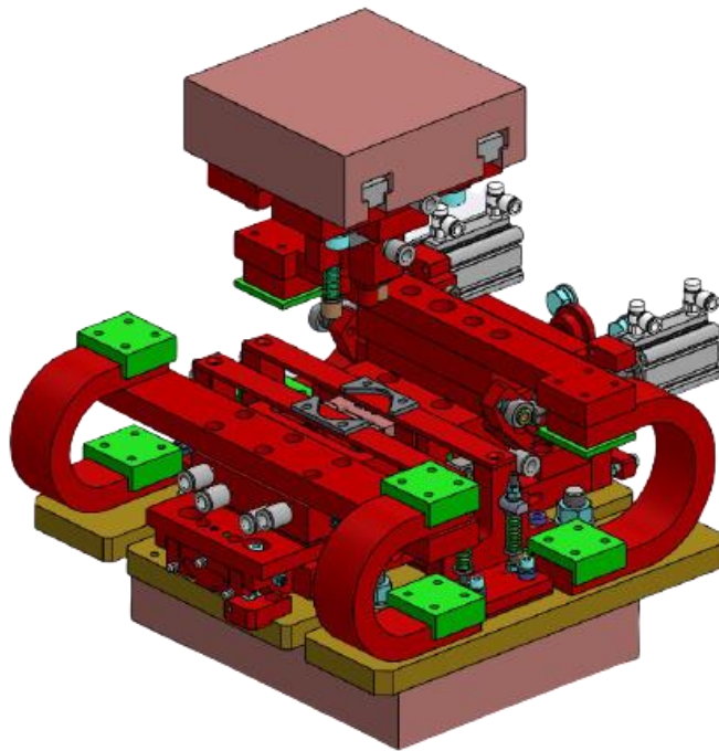
HOT RIVETING JIG.
