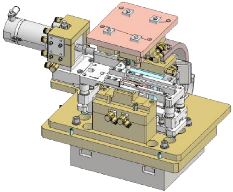
HOT RIVETING JIG.
